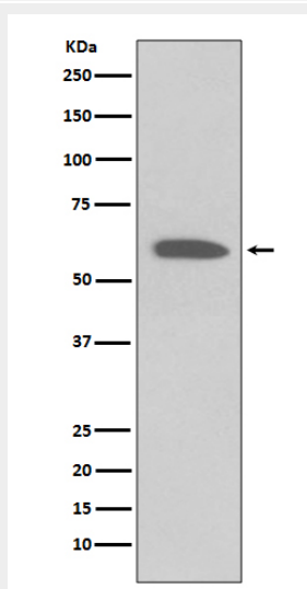
Western blot analysis on 2 NIH/3T3 cell lysate treated with PDGF using Phospho-Akt(Ser473) Antibody.
